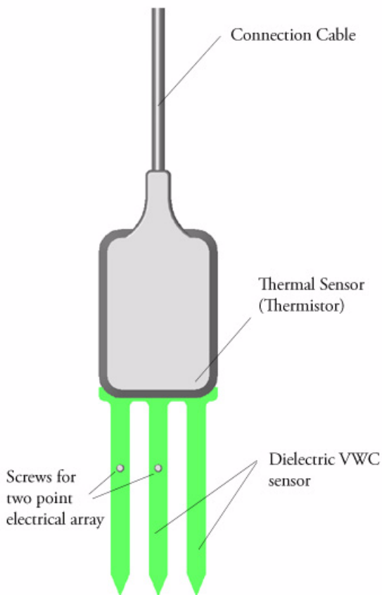
Figure 1: 5TE Components
