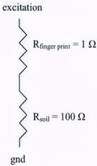
Figure 3a: Simplified circuit of contaminated probe in low EC (high resistance) soil. R_{\text{total}} = 101 \Omega , fingerprint causes 1% error.
