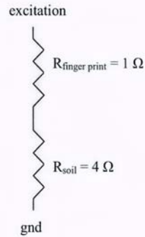
Figure 3b: Simplified circuit of contaminated probe in high EC (low resistance) soil. R_{\text{total}} = 5 \Omega , fingerprint causes 25% error
